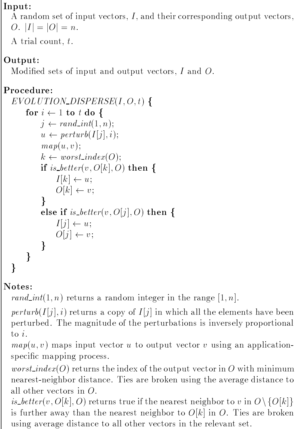
Figure 4: An evolutionary dispersion heuristic.
