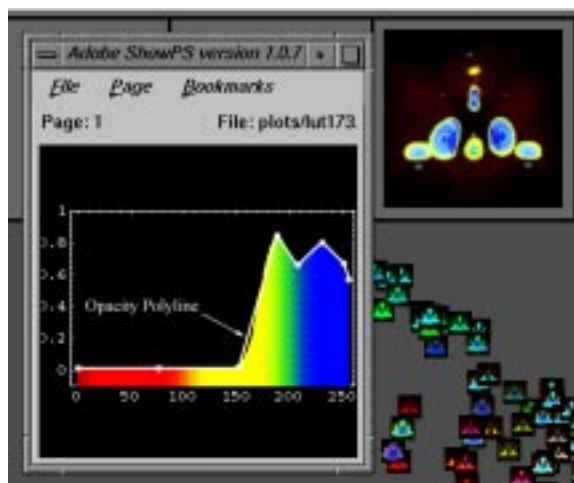
Figure 3: Pop-up display depicting transfer functions.
