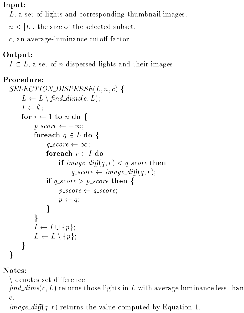
Figure 1: A selection-based dispersion heuristic.
