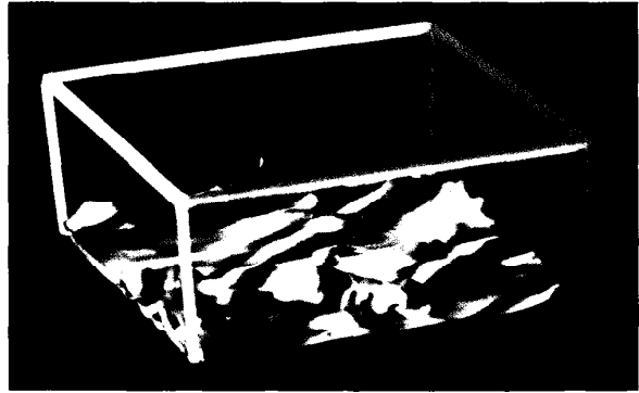
Figure 7. Volume-rendered image of the streamwise velocity component. The vertical velocity is solid texture-mapped onto the stream component, showing regions of turbulence generation in red and blue.
